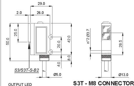
S3T - M8 CONNECTOR
