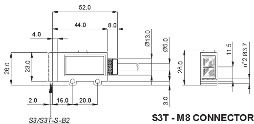
S3T - M8 CONNECTOR
