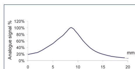
Coaxial polarized retroreflex for transparents - T53
