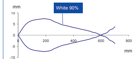
Diffuse proximity
