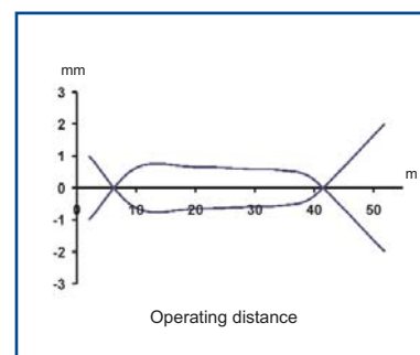
Fixed focus proximity - 50 mm Detection area
