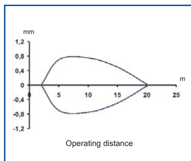
Fixed focus proximity - 20 mm Detection area
