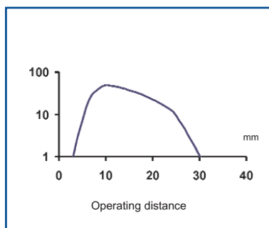
Fixed focus proximity - 30 mm Excess gain
