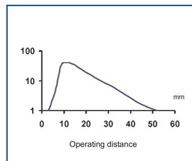
Fixed focus proximity - 50 mm Excess gain
