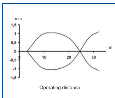
Fixed focus proximity - 30 mm Detection area
