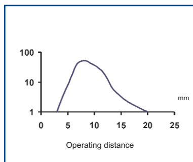
Fixed focus proximity - 20 mm Excess gain
