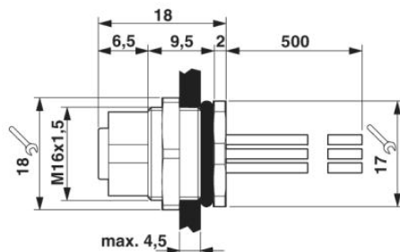
M12 flush-type socket
