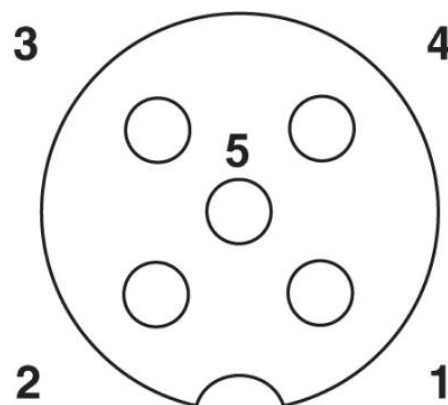
Connector pin assignment for M12 socket, 5-pos.
