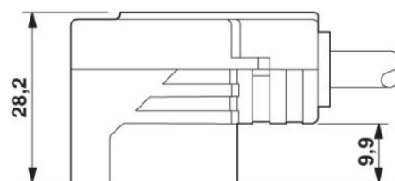
Valve connector, type AD, side view
