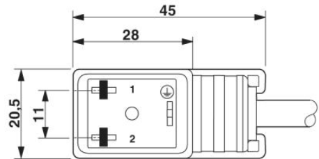
Valve connector, type BI
