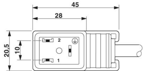
Valve plug, type B
