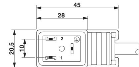
Valve plug, type B
