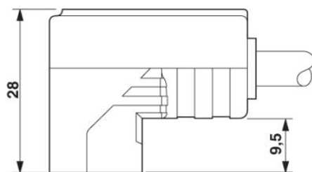
M12 x 1 male connector, angled
