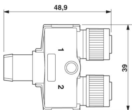
Y distributor, 2 x socket M12 x 1
