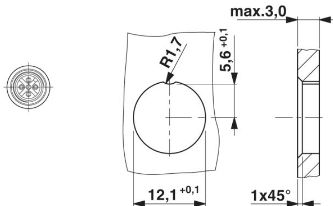
Housing cutout for M12 fastening thread, mounting panel with feed-through hole
