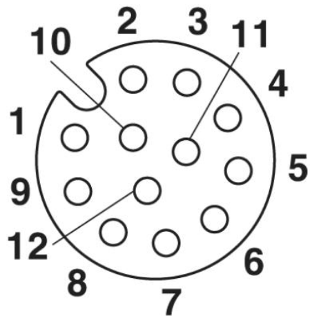
Pin assignment M12, 12-pos., female side view
