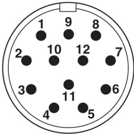
Connector pin assignment M23 plug, 12-pos., pin side view
