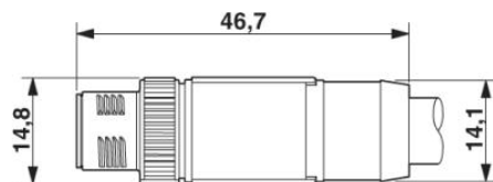
M12 SPEEDCON connector, straight, shielded
