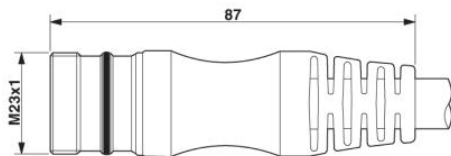
M23 plug, straight, shielded
