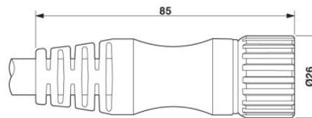
M23 socket, straight, shielded
