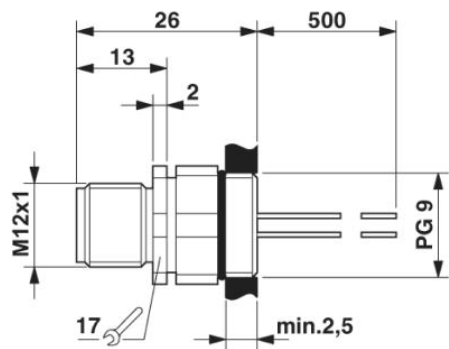
M12 flush-type connector, can be positioned
