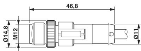
Dimensioned drawing
