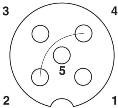
Pin assignment socket M 12, 3-pos. + PE
