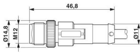
M12 x 1 male connector, straight
