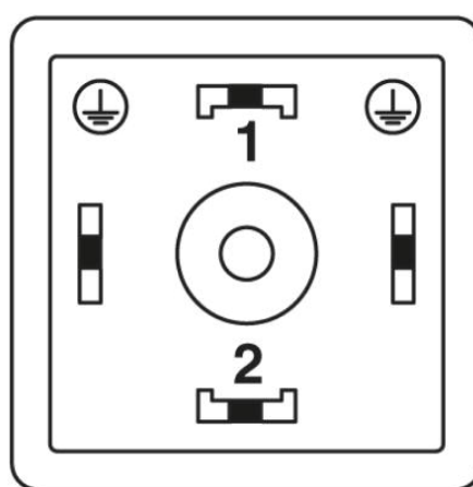
Valve connector pin assignment, type A
