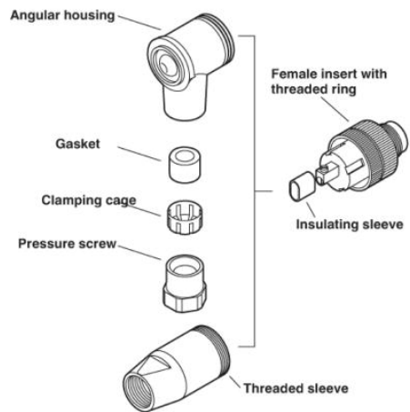
Male/Female M12
