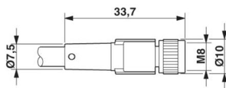
Socket M8 x 1, straight, shielded
