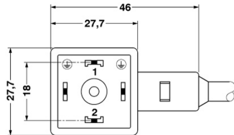
Valve plug, type A, flat
