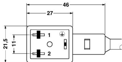
Valve connector, type BI, flat
