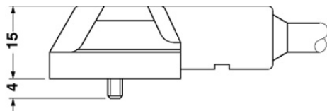
Valve connector, type BI, flat
