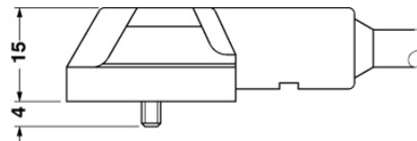
Valve connector, type C, flat
