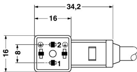
Valve connector, type C, flat
