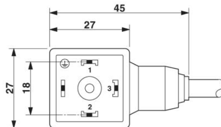
Valve plug type AD
