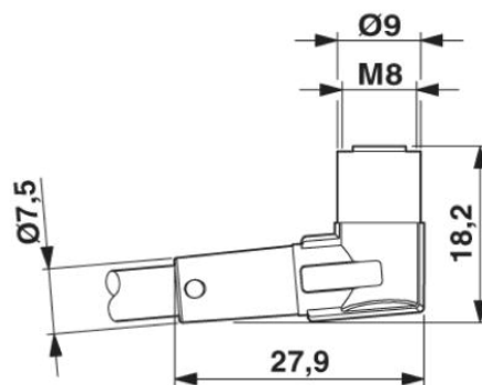
M8 socket, snap-in, angled
