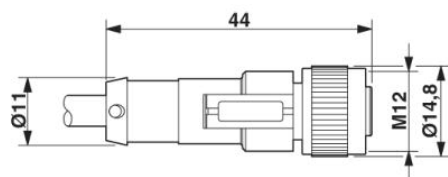
Dimensioned drawing
