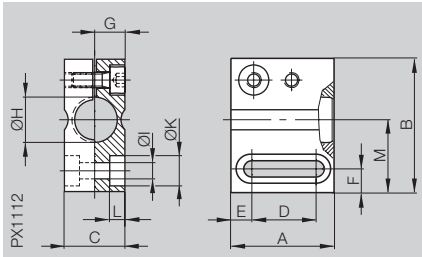
Mounting clamp with positive stop (material: Al)
